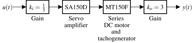
Figure 2. Block diagram for input-output data acquisition.
