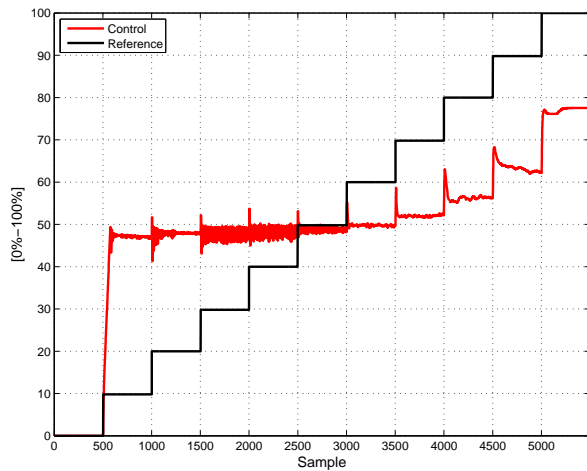
Figure 10. Control effort for the linear controller (6).
