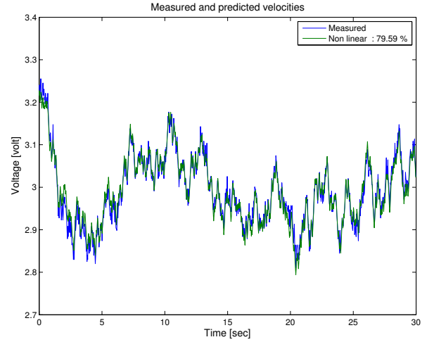
Figure 6. Fit between measured and predicted velocities (nonlinear model (1)).
