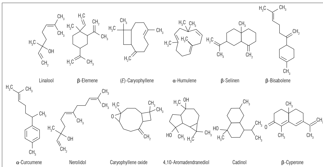
Figure 1. Chemical structure of the main compounds found in the EOs of P. coruscans , P. ottoniaefolium , and P. reticulatum . Developed in: MarvinSketch ver. 23.2 .
