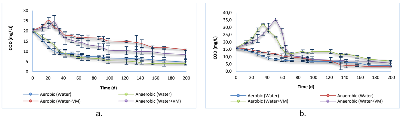
Fig. 2. Degradation of organic matter in terms of COD by aerobic and anaerobic processes. a) Behavior P1. b) P2 behavior.
